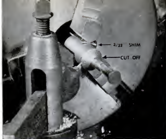
Pulley for the belt that drove the vacuum's brush is cut off, as shown above, before the remaining stub is turned off center.
